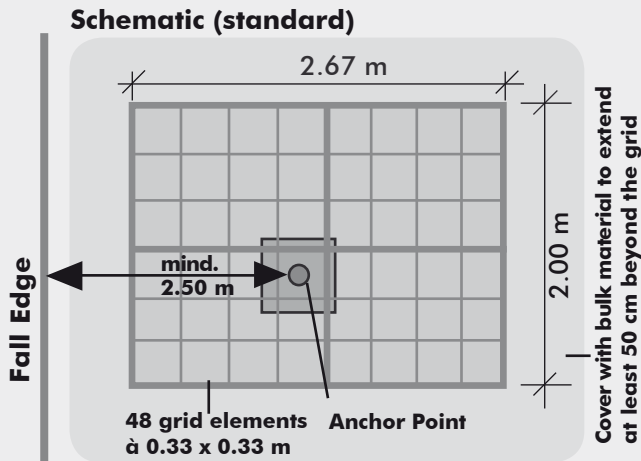
Schematic of a standard installation of the centred Anchor Point with the four pre-assembled grids (à 1.00 × 1.33 m).
